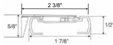
Cord Lock Rail
