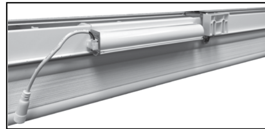
Snap-On external battery for shades under 36" in width. Spacer block also shown, required for outside mount.
